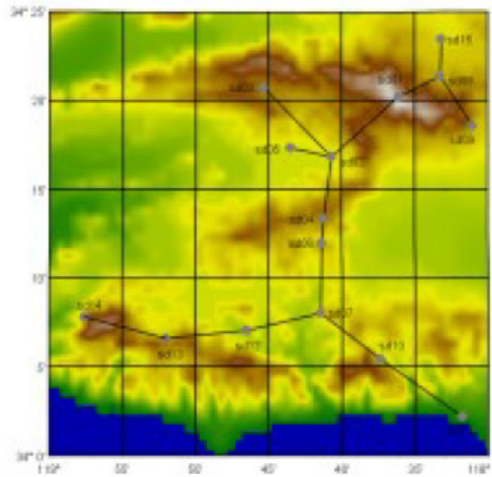
Pathloss 4.0 Transmission Link Planner
